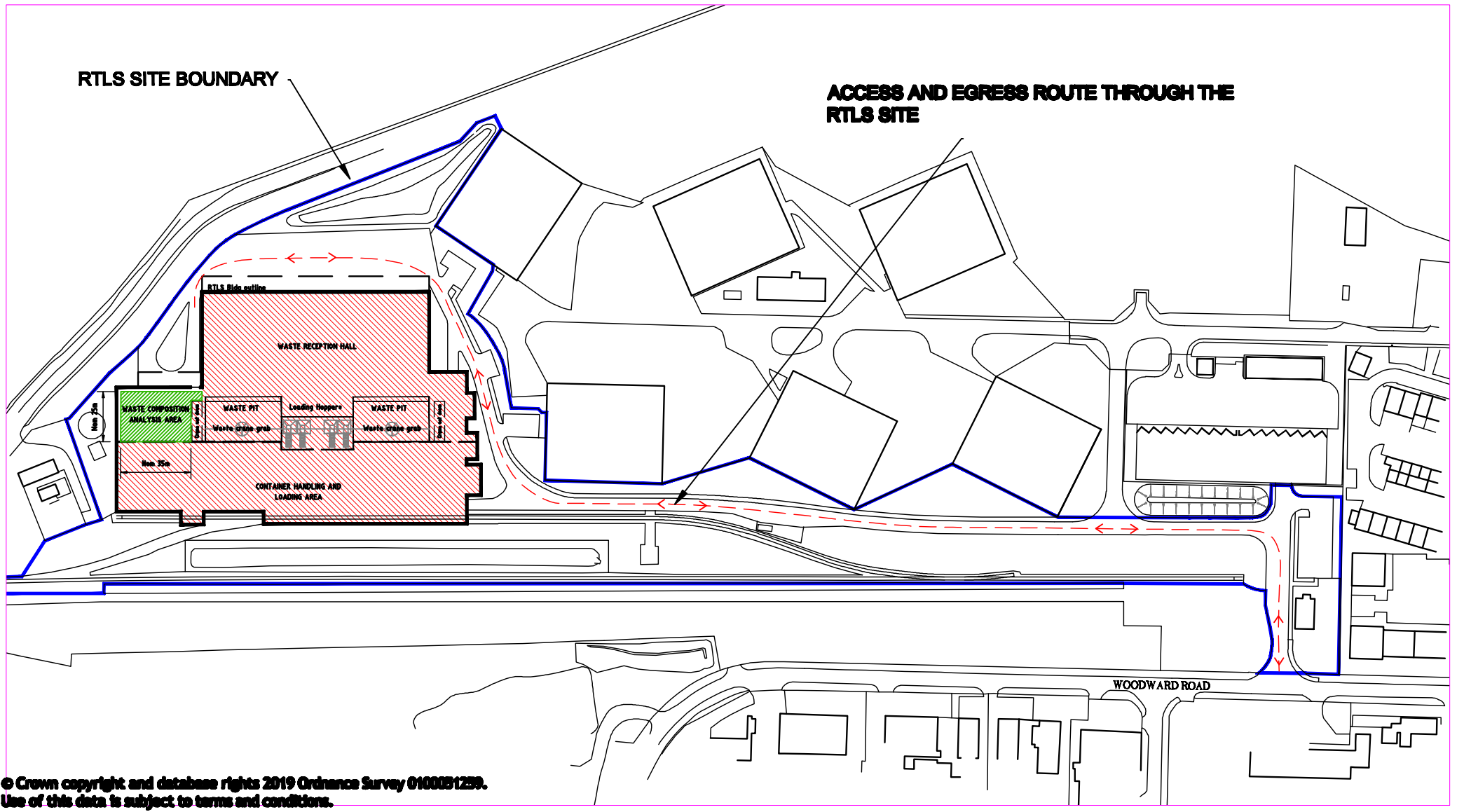
RAIL TRANSFER LOADING STATION - SITE LAYOUT Scale 1:2500
