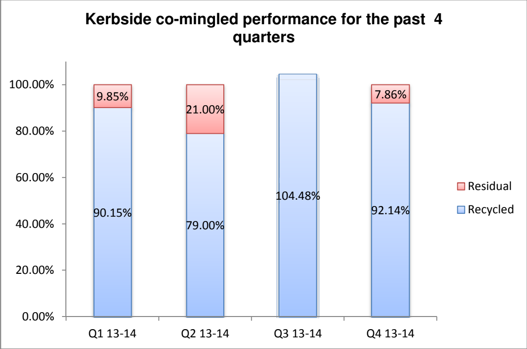
Fig 3: KCM Performance
